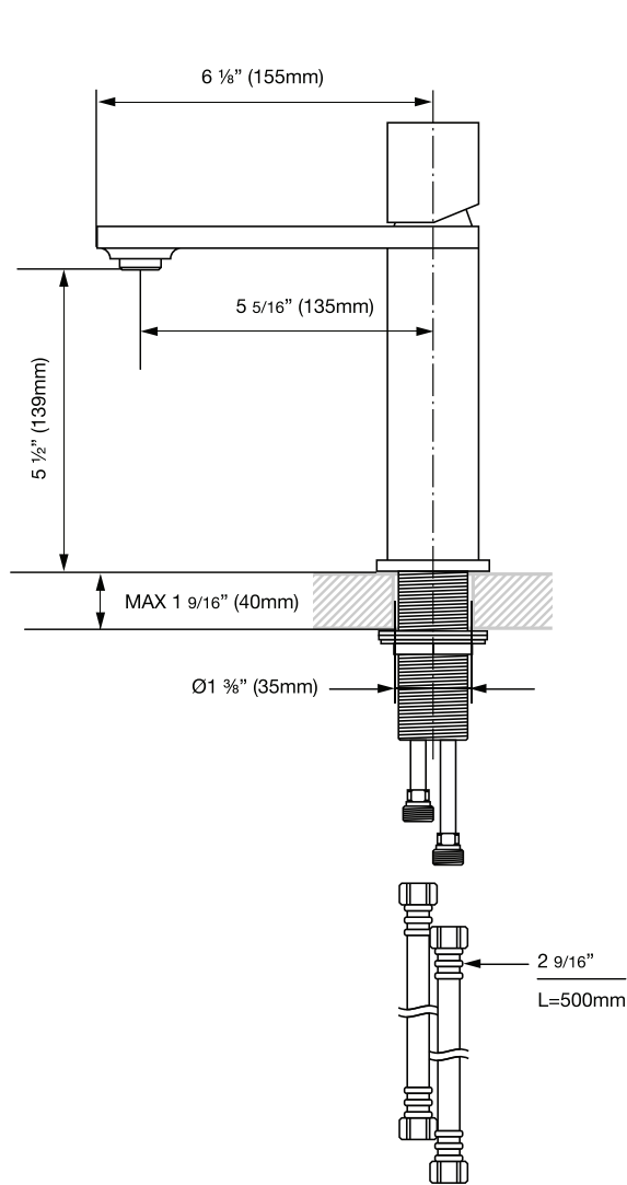
FRONT VIEW
